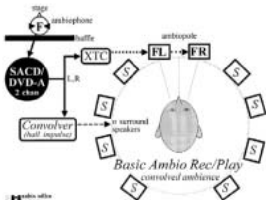
Fig. 3. Two Channel Ambiohonic System
