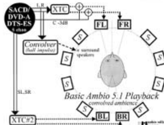
Fig. 4. Ambiohonic Playback of 5.1 Material
