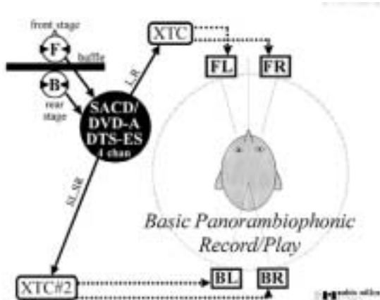
Fig. 5 Panorambiophonics Delivers Full Circle Localization via 4 Channels and Speakers
