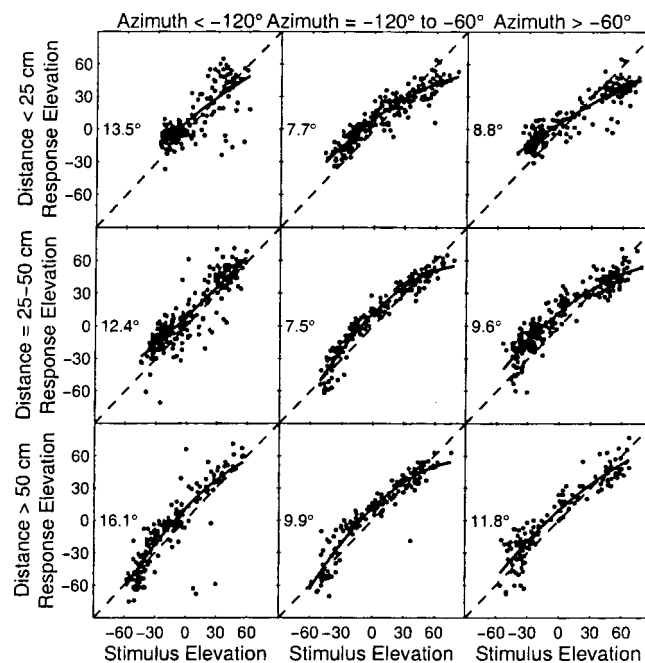
FIG. 5. The nine panels show raw elevation stimulus and response locations for subject KMY, a typical subject in the experiment. Azimuths were divided into regions less than -120^\circ , from -120^\circ to -60^\circ , and greater than -60^\circ . Distances were divided into regions less than 25 cm, from 25 to 50 cm, and greater than 50 cm. A dashed line represents correct responses. The BCRMS elevation error is shown at the left side of each panel, and the solid line represents the best second-order polynomial fit of the stimulus data to the response locations. Note that the stimuli range from approximately -45^\circ to 80^\circ in elevation. The data are limited at low elevations because the subject's torso and the chin rest prevented placement at some source locations. For example, low elevations are particularly truncated at close distances behind the subject where the neck and back prevented placement at low elevations.
