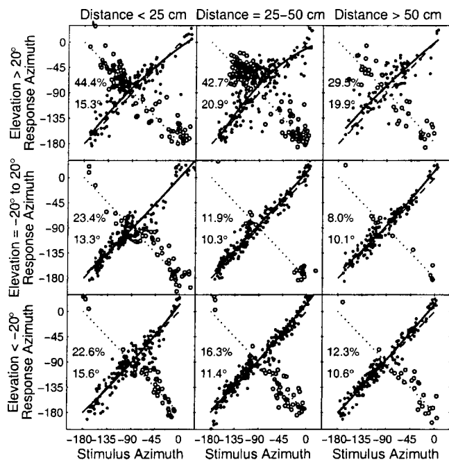
FIG. 2. Raw azimuth stimulus and response data for subject CLL. The data were sorted according to source distance into three regions: closer than 25 cm; from 25–50 cm; and farther than 50 cm. Similarly, the data were sorted by source elevation into three regions: above 20°; between –20° and 20°; and below –20°. Columns represent distance, increasing left to right, and rows represent elevation. The solid line is the second-order polynomial function of the stimulus location that best fits the response location. At the left of each panel are two numbers. The upper number is the percentage of front–back reversals (represented by open circles) in the region. The lower number is the BCRMS for all nonreversed responses in the panel (see the text). The dashed line represents “correct” responses, while the dotted line represents “perfect” reversals. Note that this subject exhibited an atypically large number of front–back reversals.
