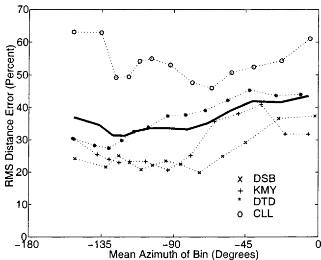
FIG. 8. rms percent distance error as a function of azimuth. Each subject's responses were sorted by azimuth into 13 overlapping bins containing 14% of the total number of trials. Then, the rms percentage distance error (uncorrected for bias) calculated in each bin was plotted as a function of the mean azimuth location in each of the 13 bins. The solid line shows the average of the percent rms errors calculated for each of the four subjects.
